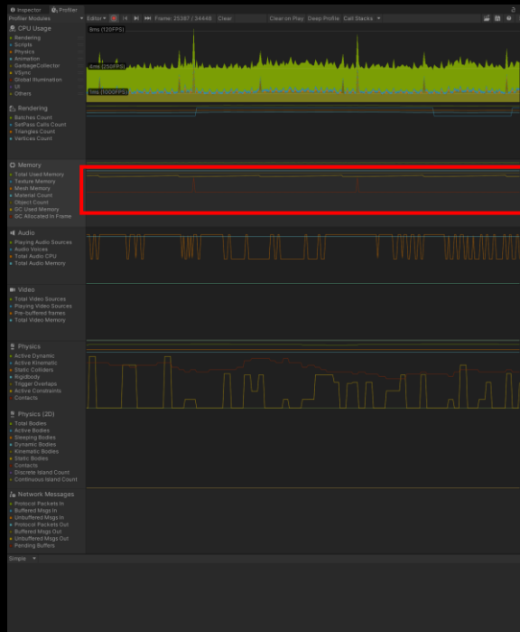
Object Pooling
