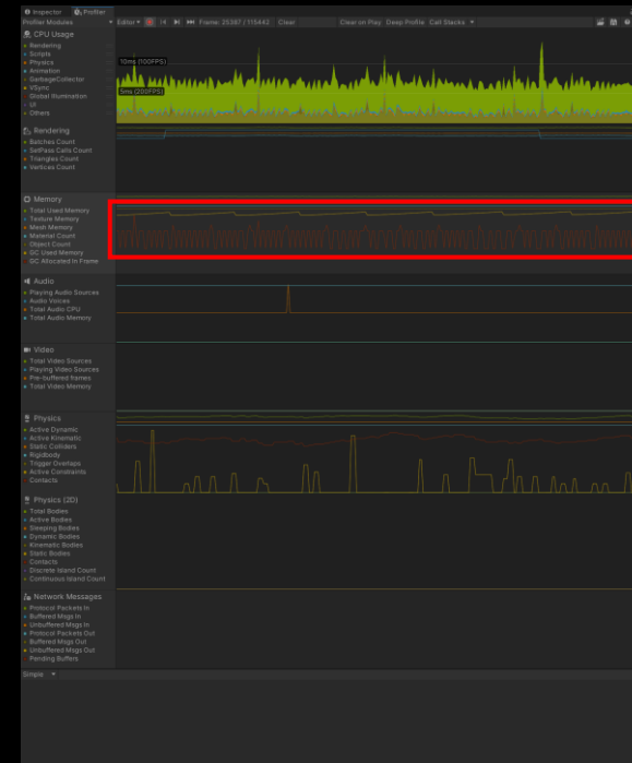
Instantiate & Destroy
